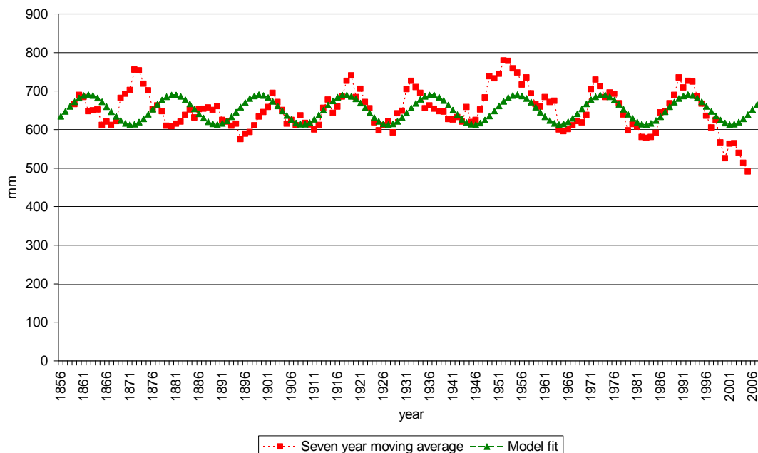
Melbourne Rainfall - model fit vs seven year moving average
