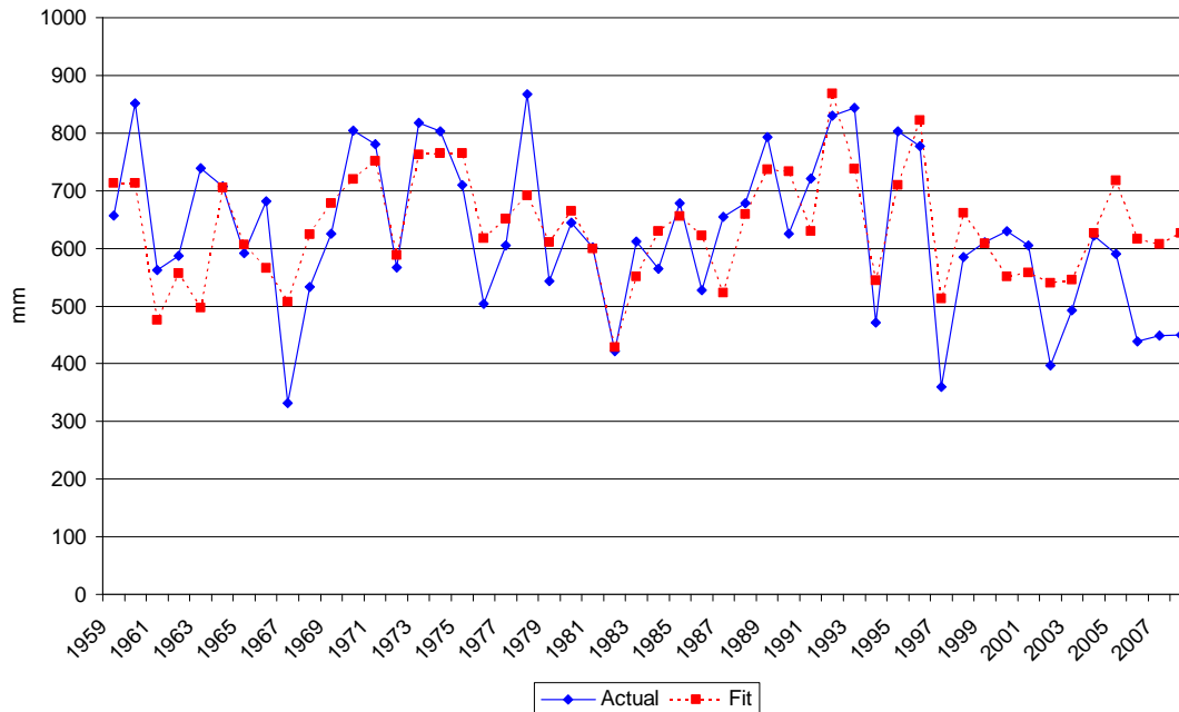
Melbourne Rainfall and Model Incorporating the Lunar Node Cycle and Indian Ocean Dipole source: BOM, foreseechange
